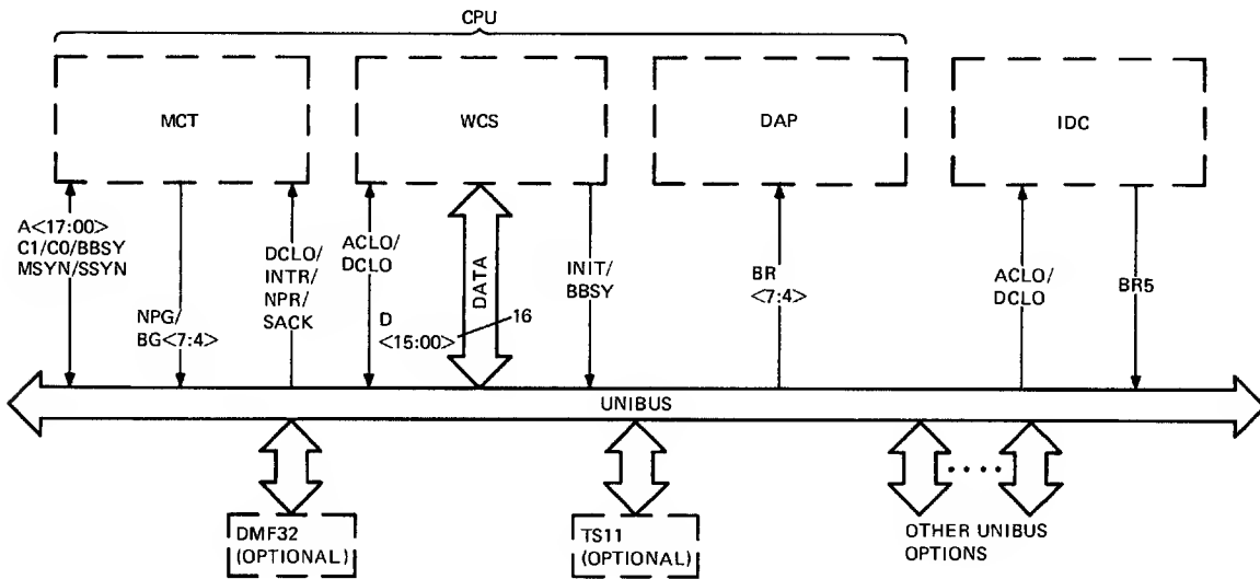
Figure 1-8 VAX-11/730 UNIBUS
